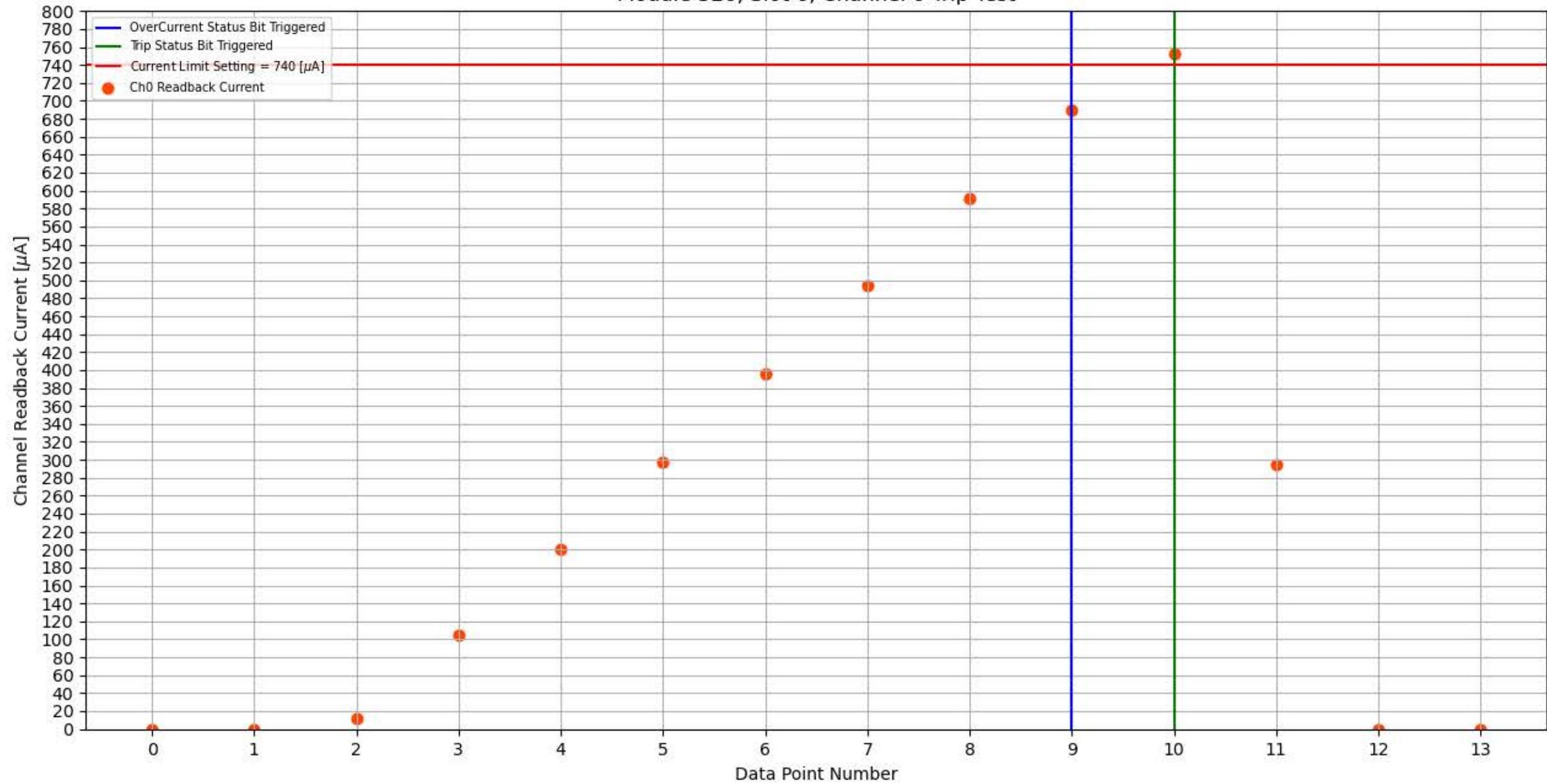
Module 326, Slot 6, Channel 0 Trip Test
