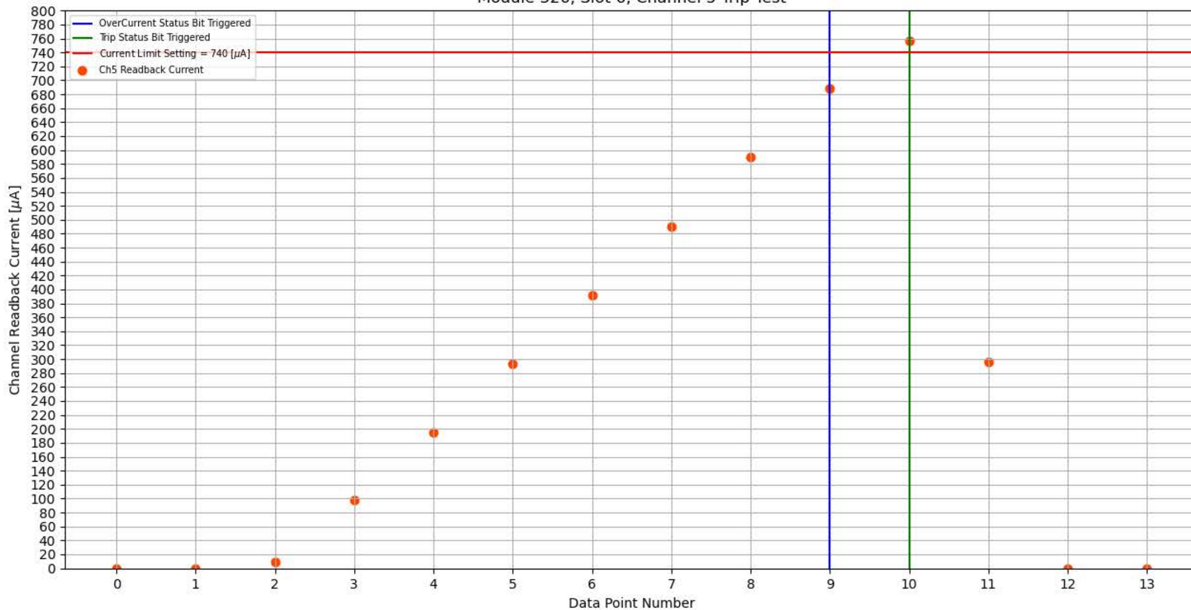
Module 326, Slot 6, Channel 5 Trip Test
