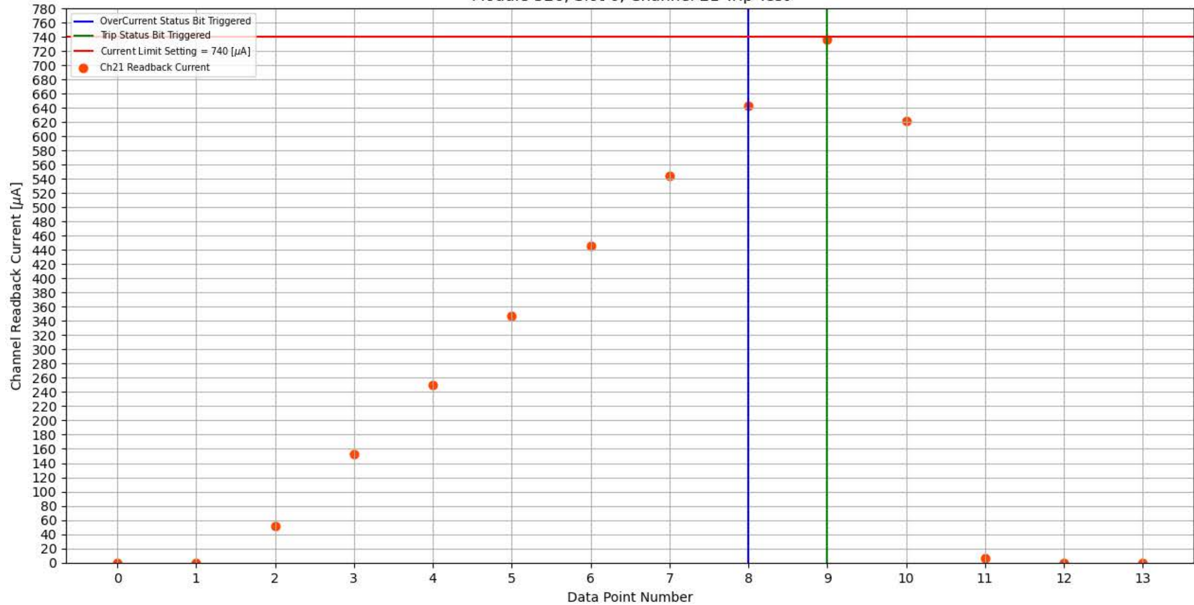
Module 326, Slot 6, Channel 21 Trip Test
