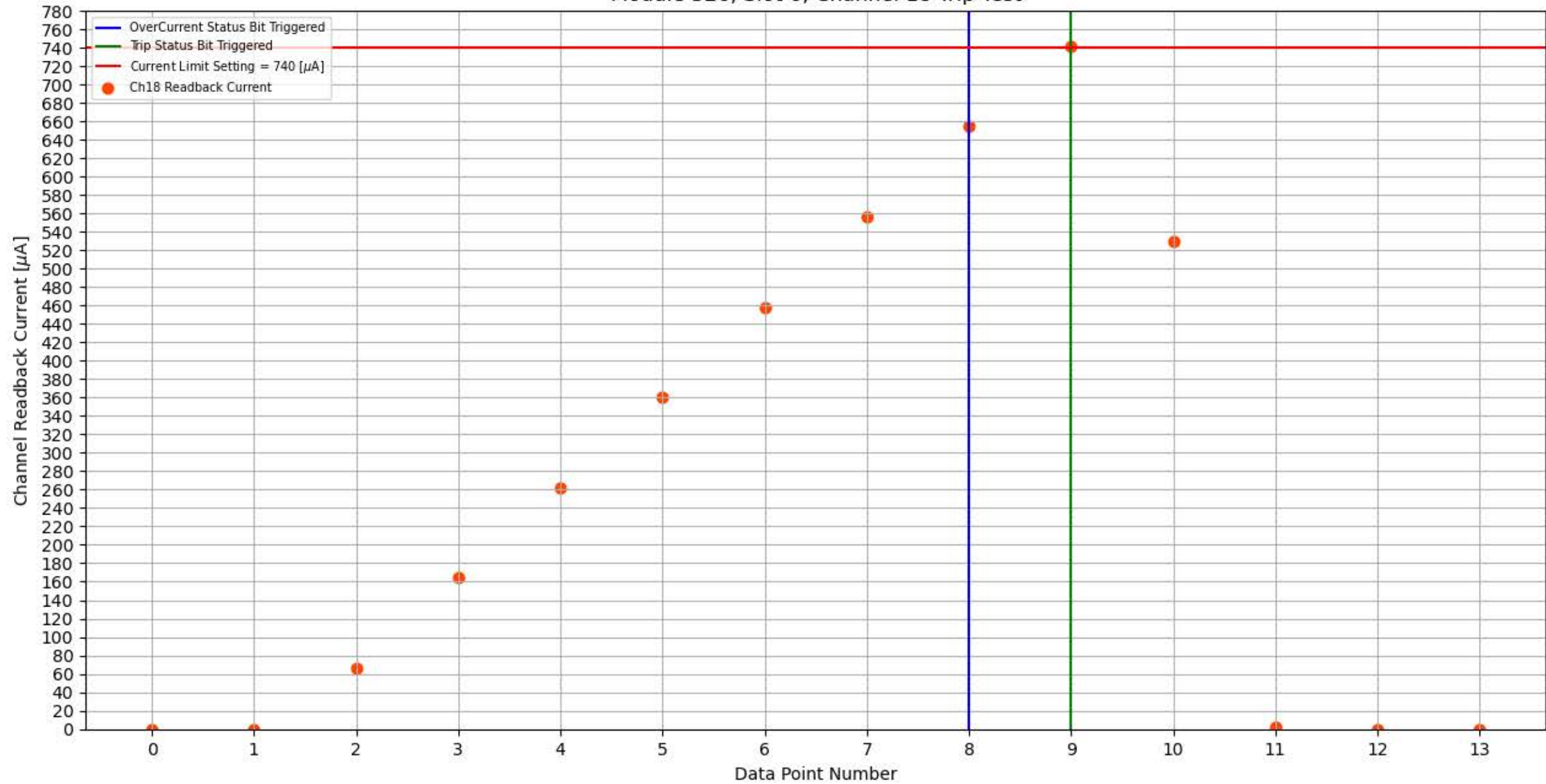
Module 326, Slot 6, Channel 18 Trip Test
