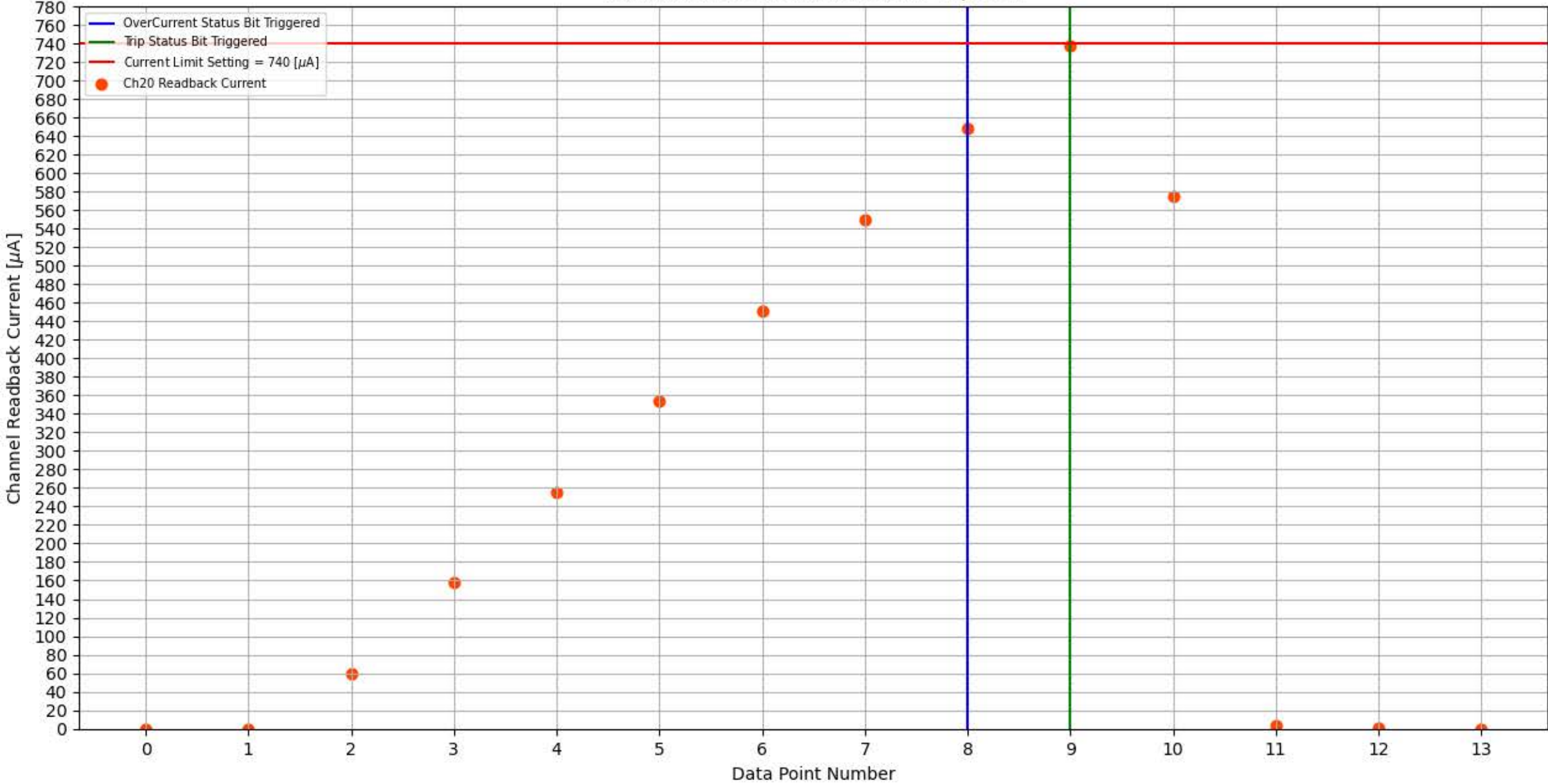
Module 326, Slot 6, Channel 20 Trip Test
