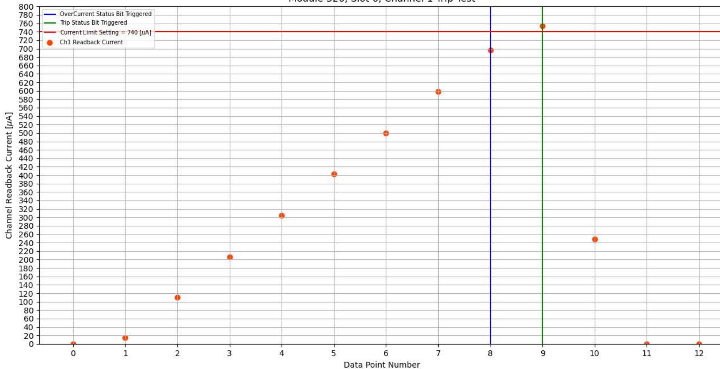
Module 326, Slot 6, Channel 1 Trip Test
