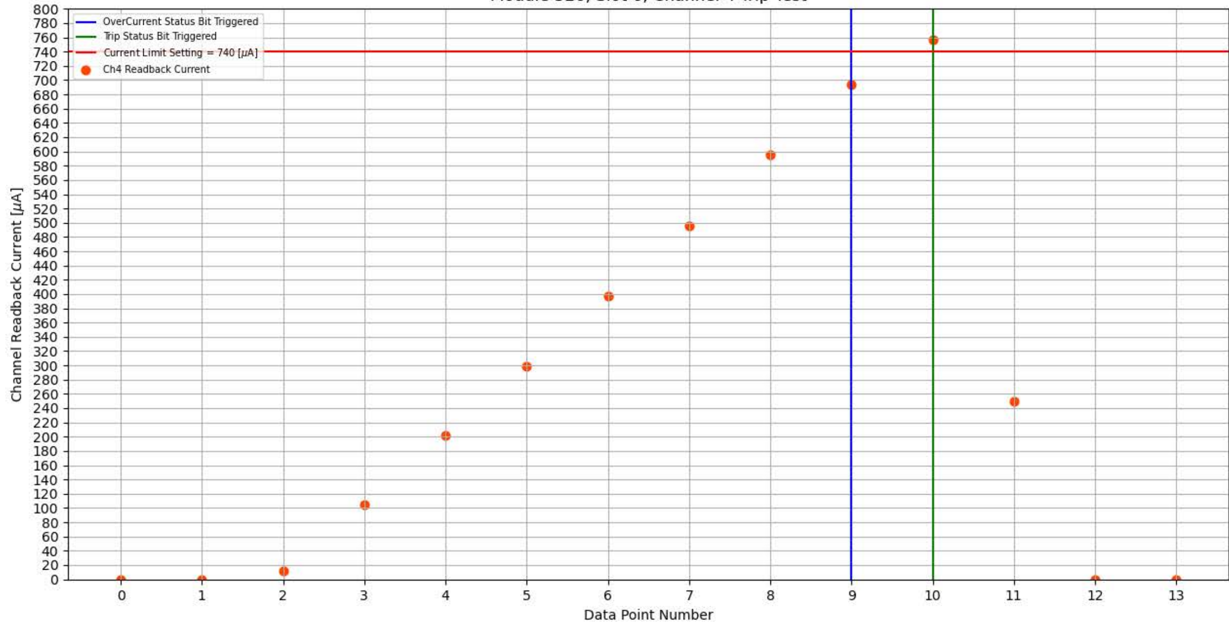
Module 326, Slot 6, Channel 4 Trip Test
