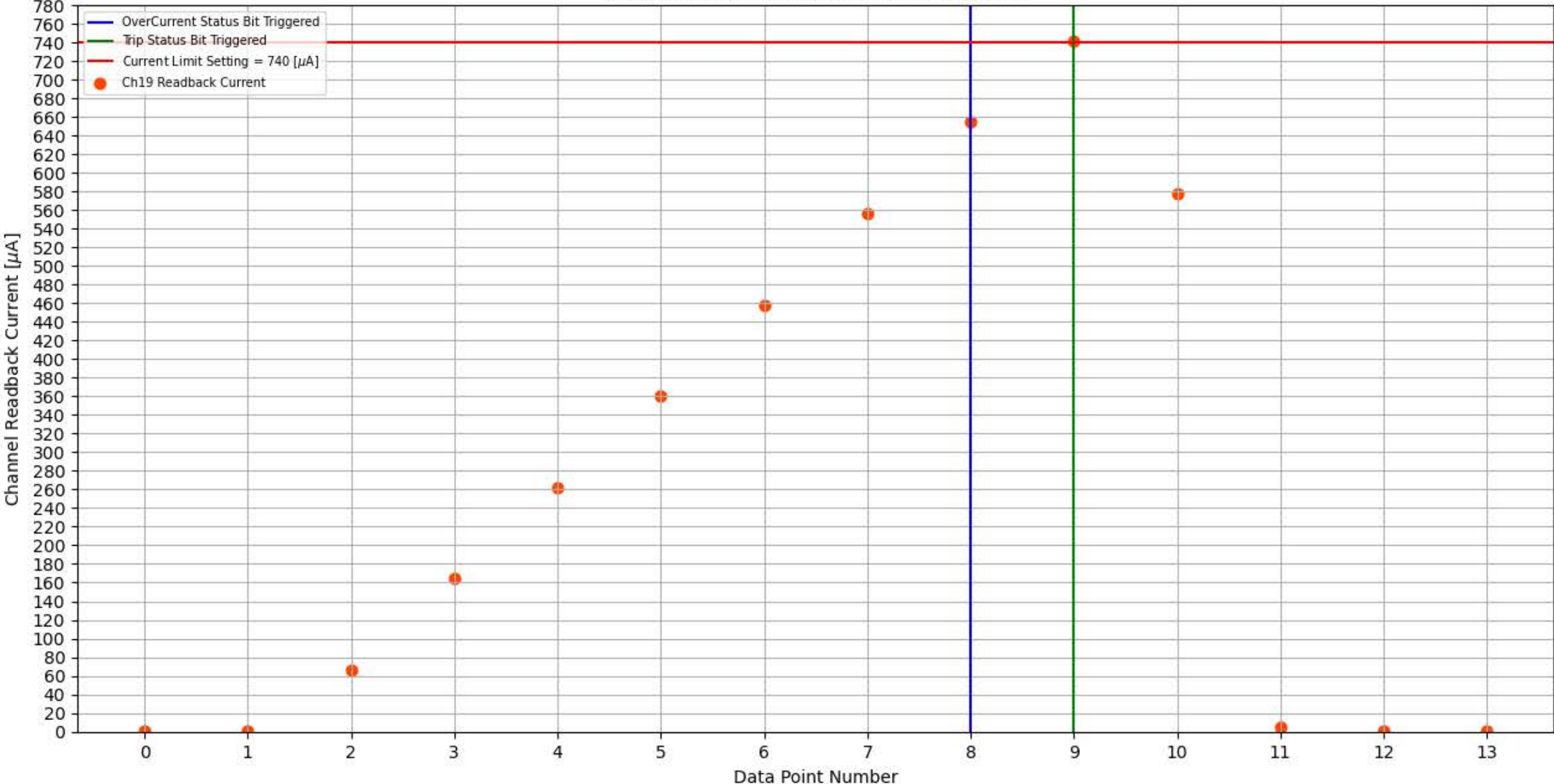
Module 326, Slot 6, Channel 19 Trip Test
