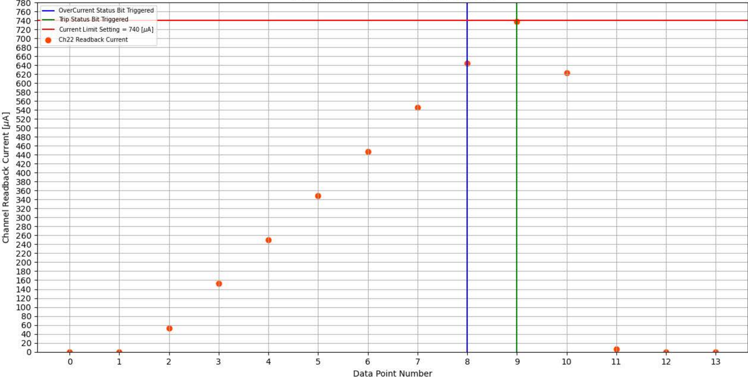
Module 326, Slot 6, Channel 22 Trip Test
