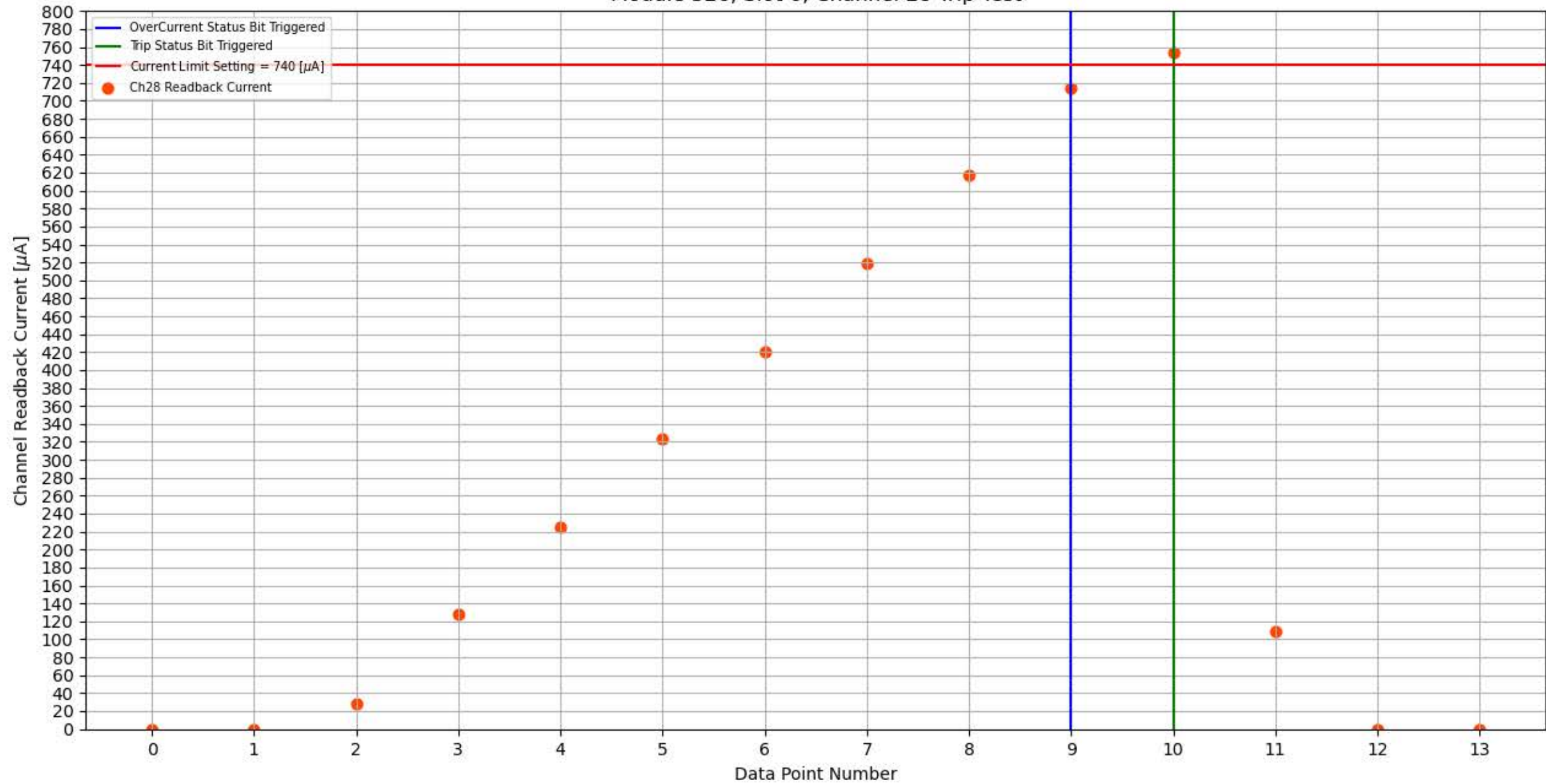
Module 326, Slot 6, Channel 28 Trip Test
