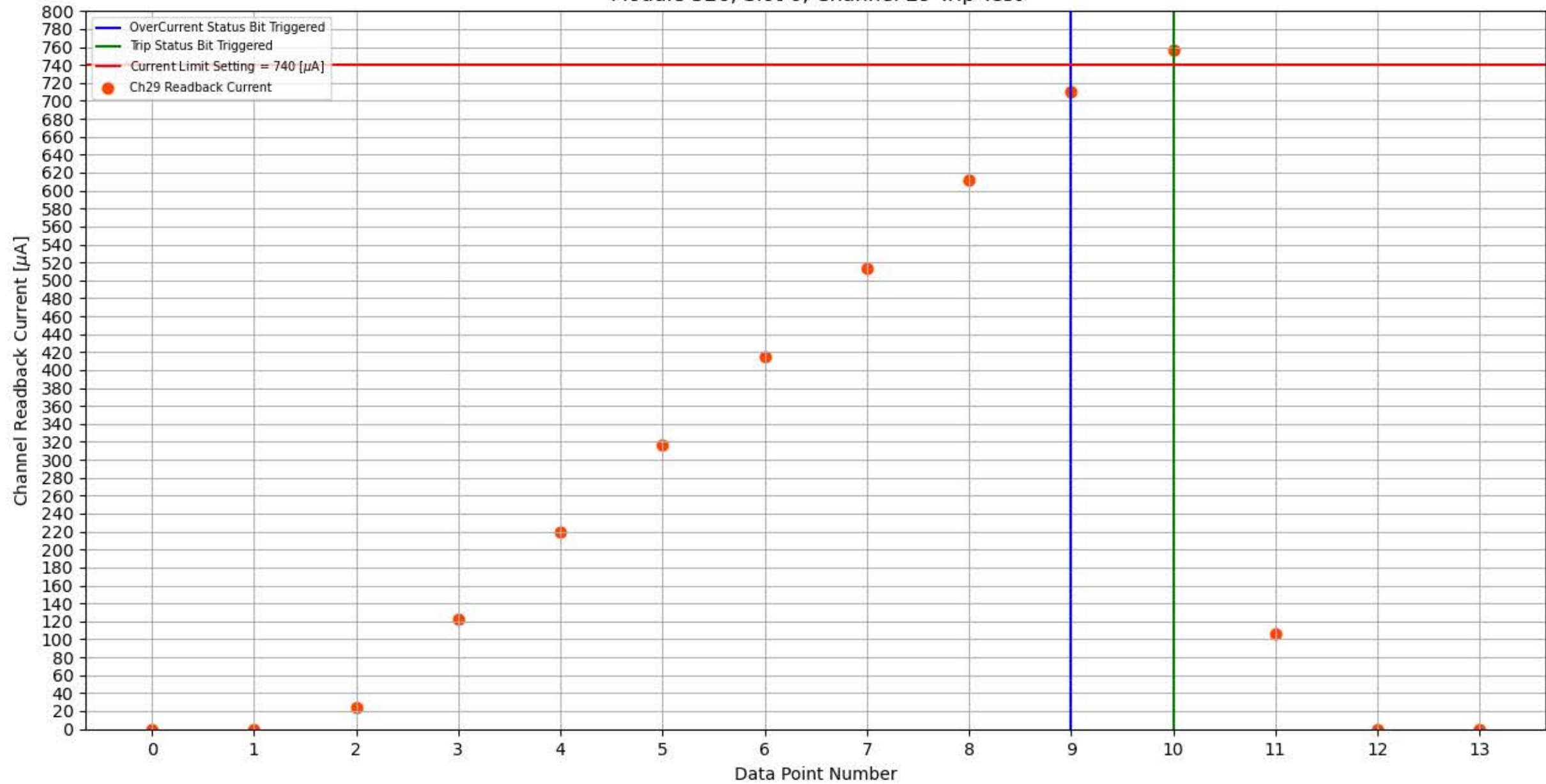
Module 326, Slot 6, Channel 29 Trip Test
