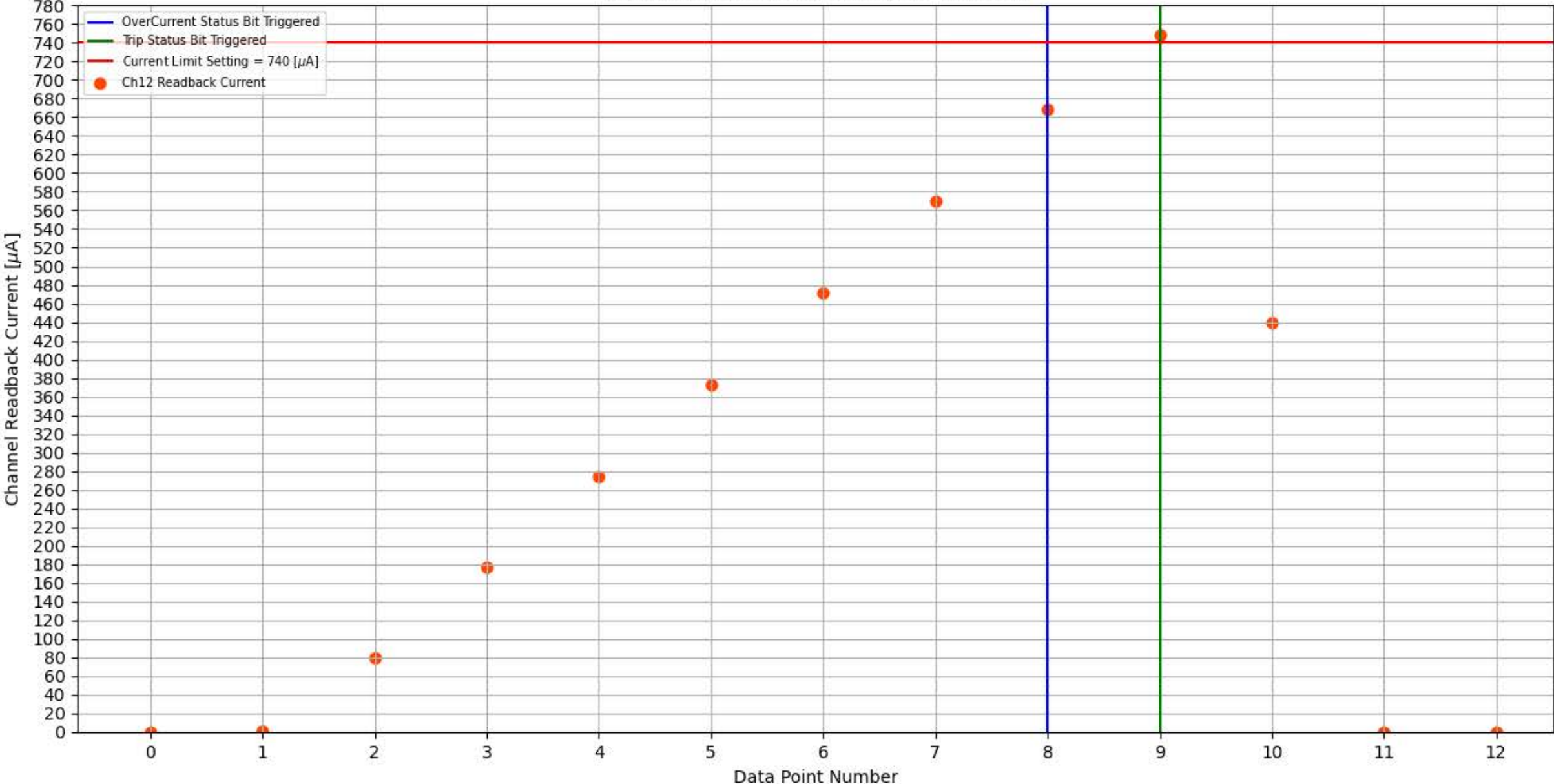
Module 326, Slot 6, Channel 12 Trip Test
