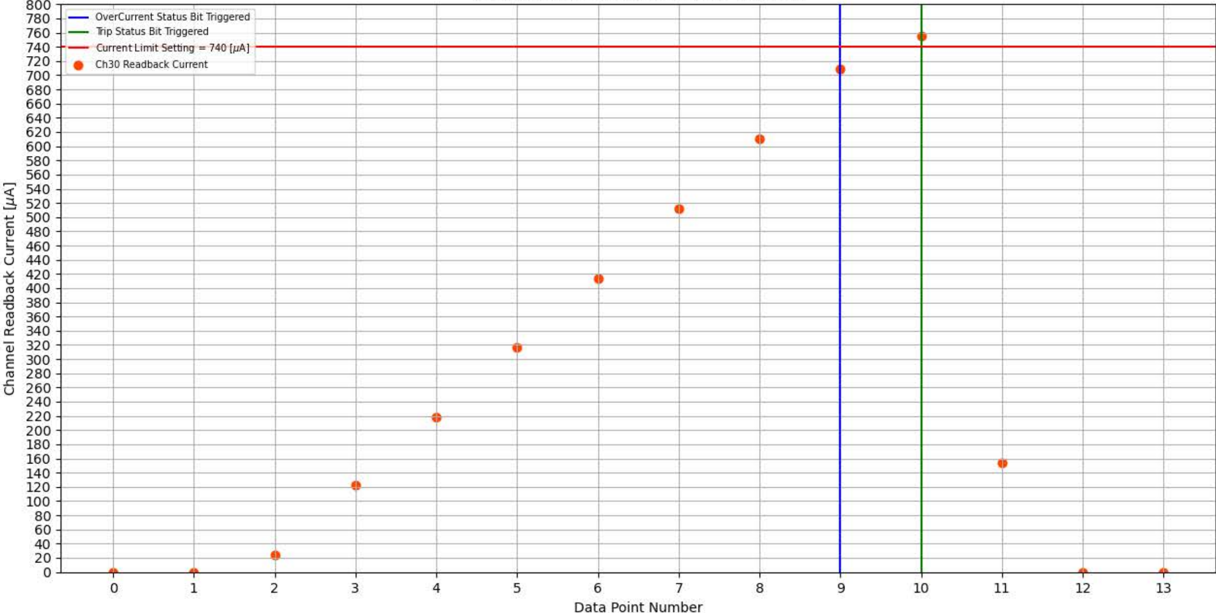
Module 326, Slot 6, Channel 30 Trip Test
