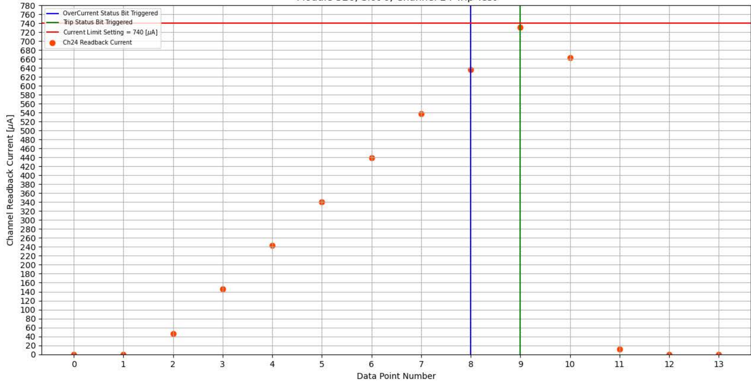
Module 326, Slot 6, Channel 24 Trip Test
