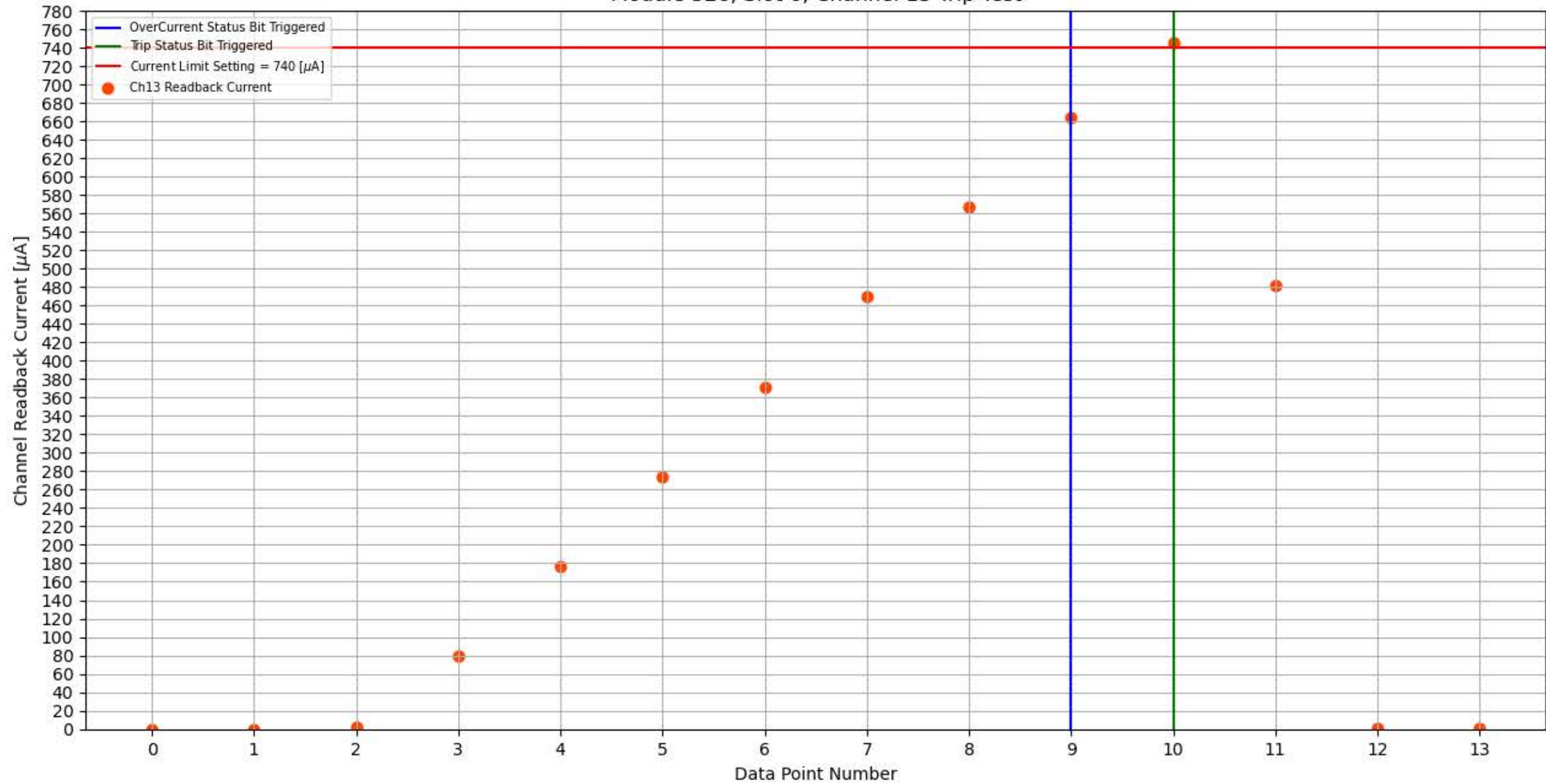
Module 326, Slot 6, Channel 13 Trip Test
