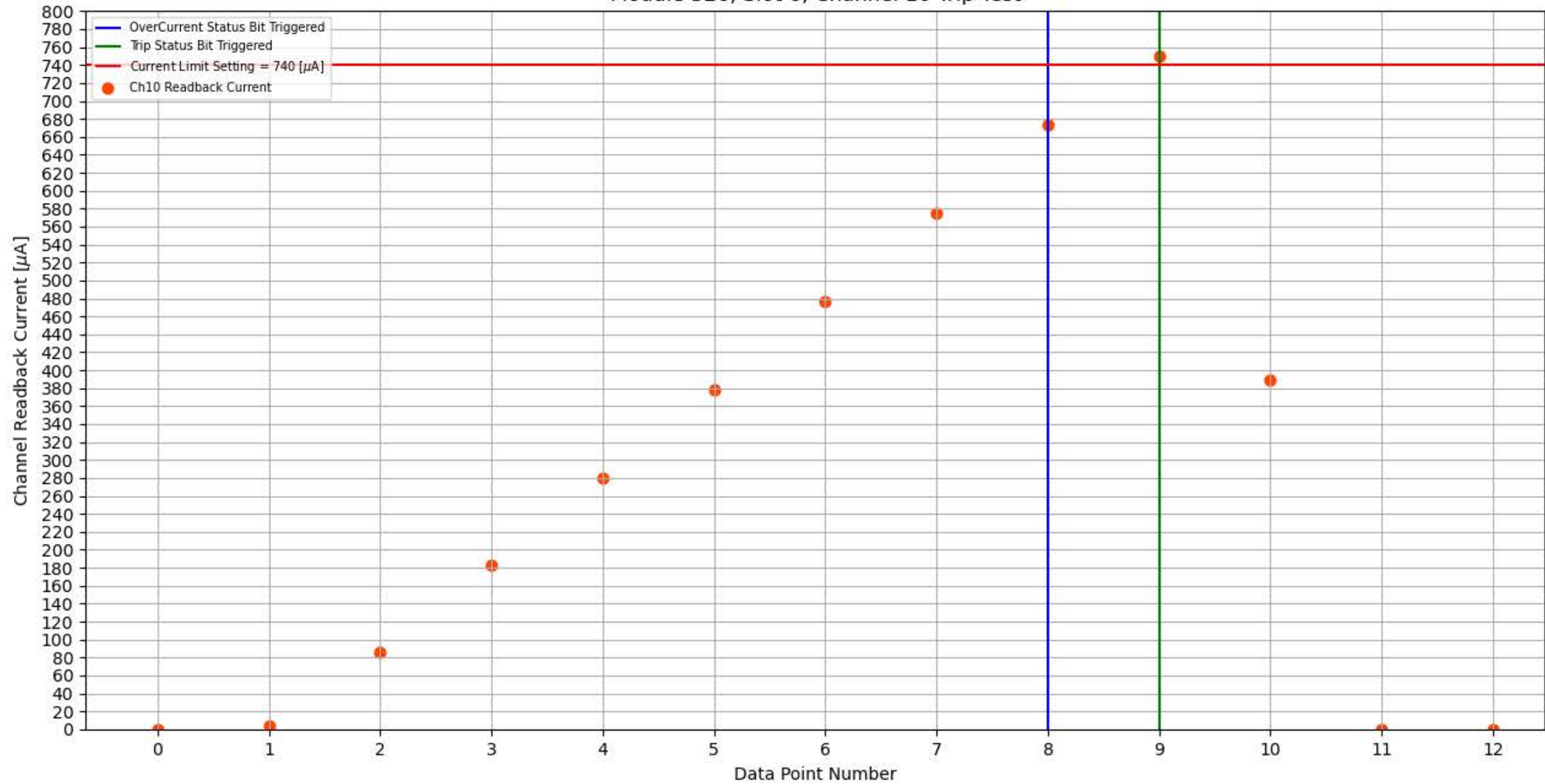
Module 326, Slot 6, Channel 10 Trip Test
