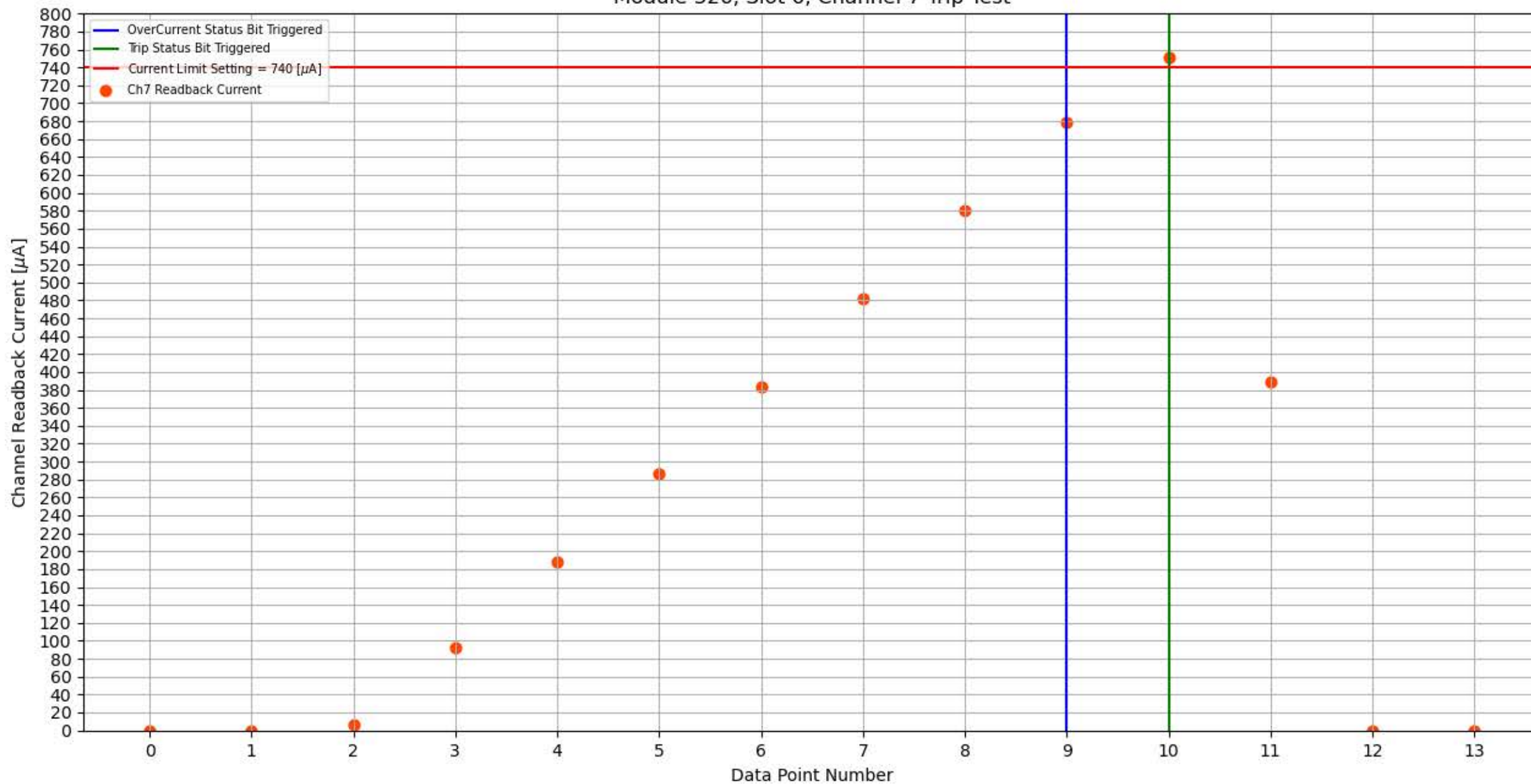
Module 326, Slot 6, Channel 7 Trip Test
