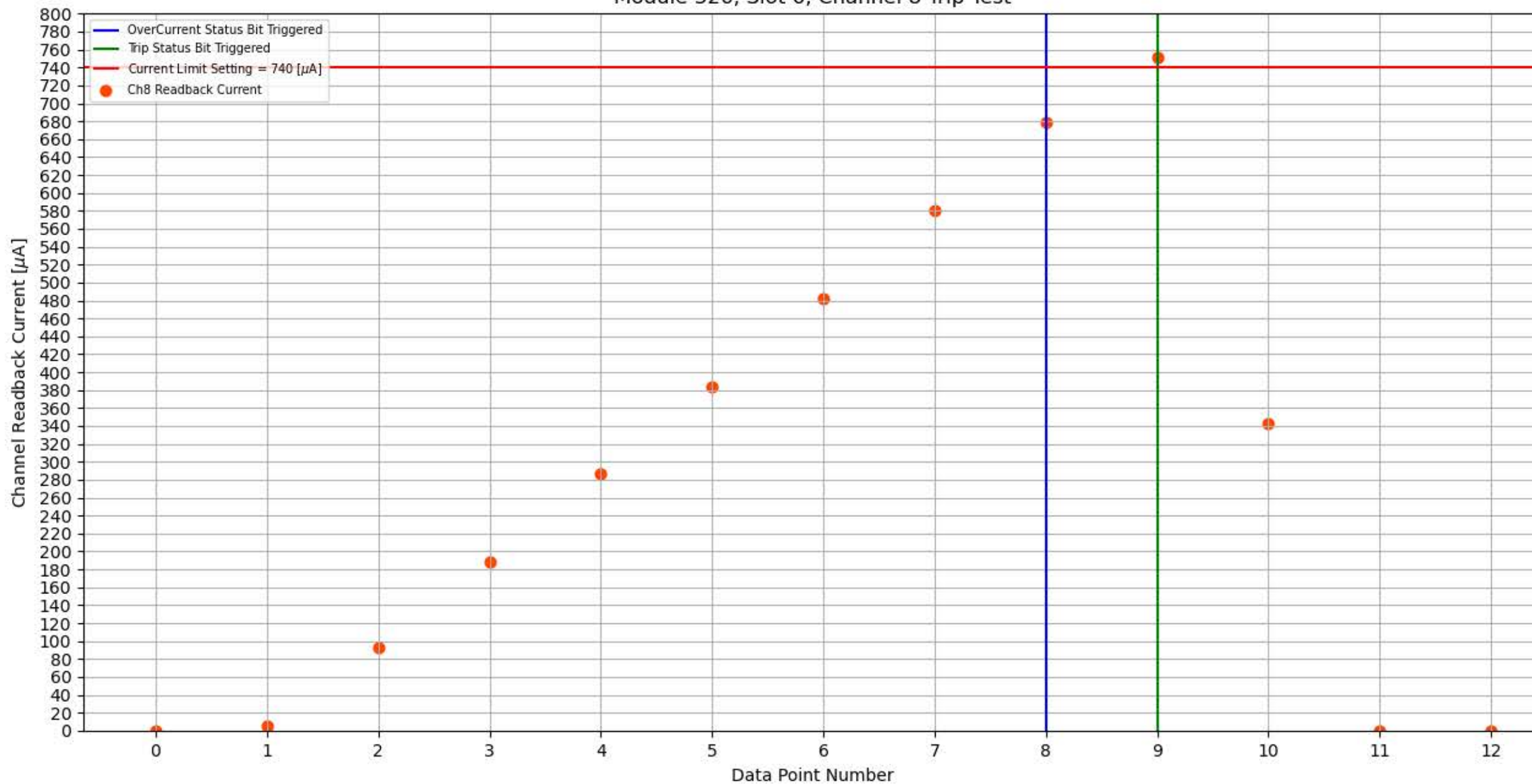
Module 326, Slot 6, Channel 8 Trip Test
