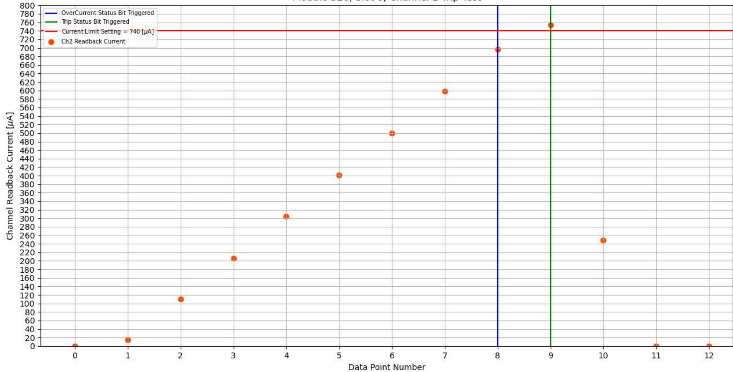
Module 326, Slot 6, Channel 2 Trip Test
