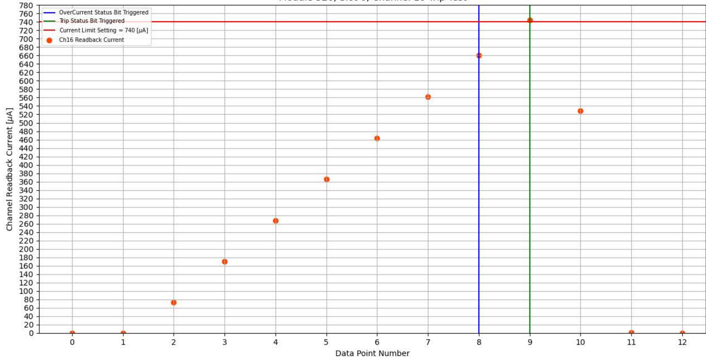
Module 326, Slot 6, Channel 16 Trip Test
