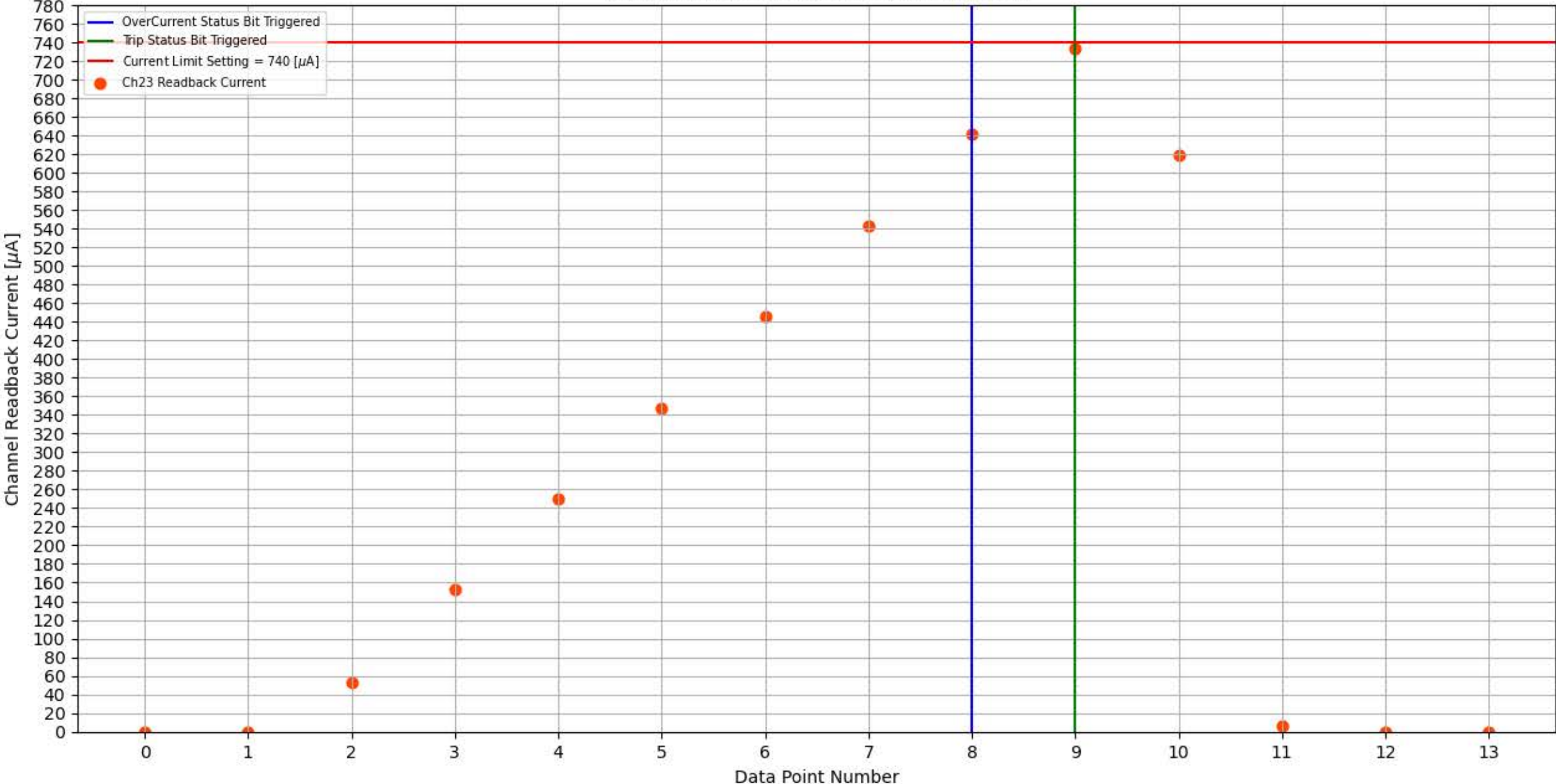
Module 326, Slot 6, Channel 23 Trip Test
