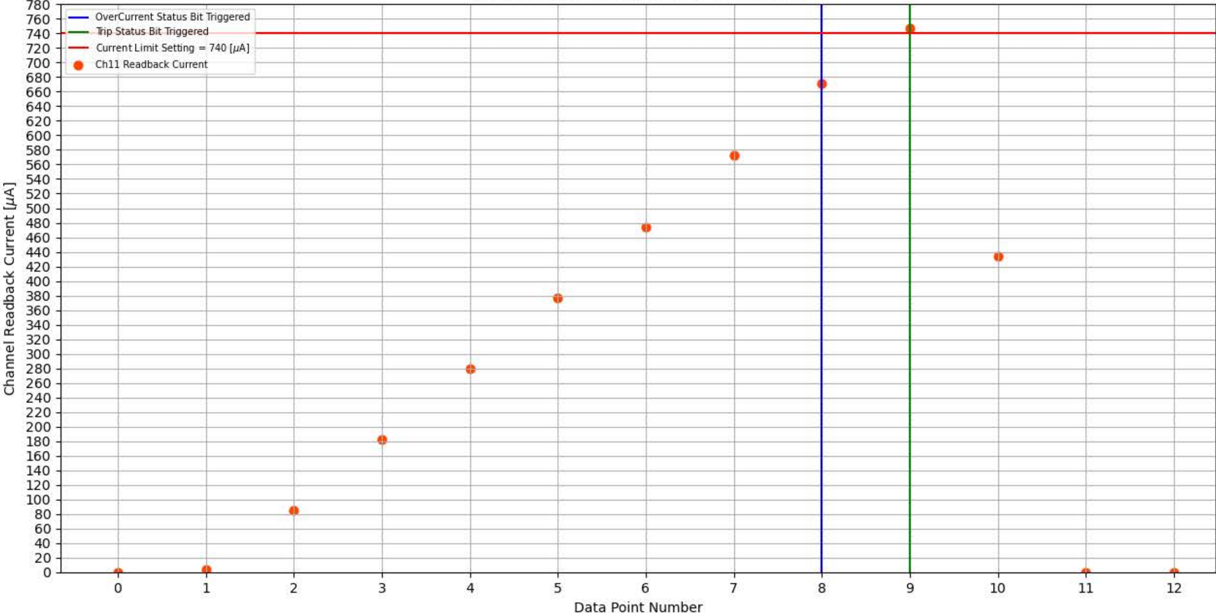
Module 326, Slot 6, Channel 11 Trip Test
