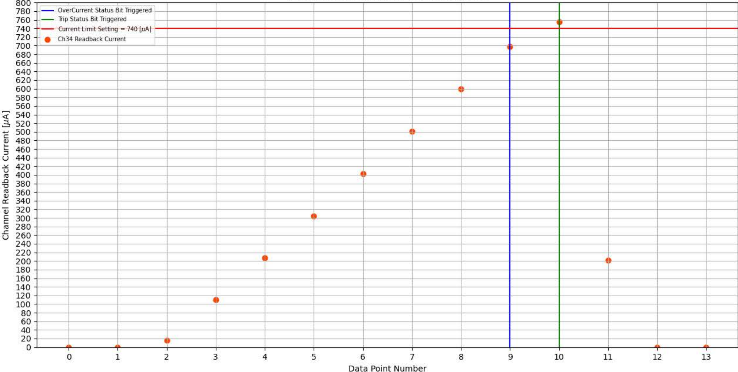
Module 326, Slot 6, Channel 34 Trip Test
