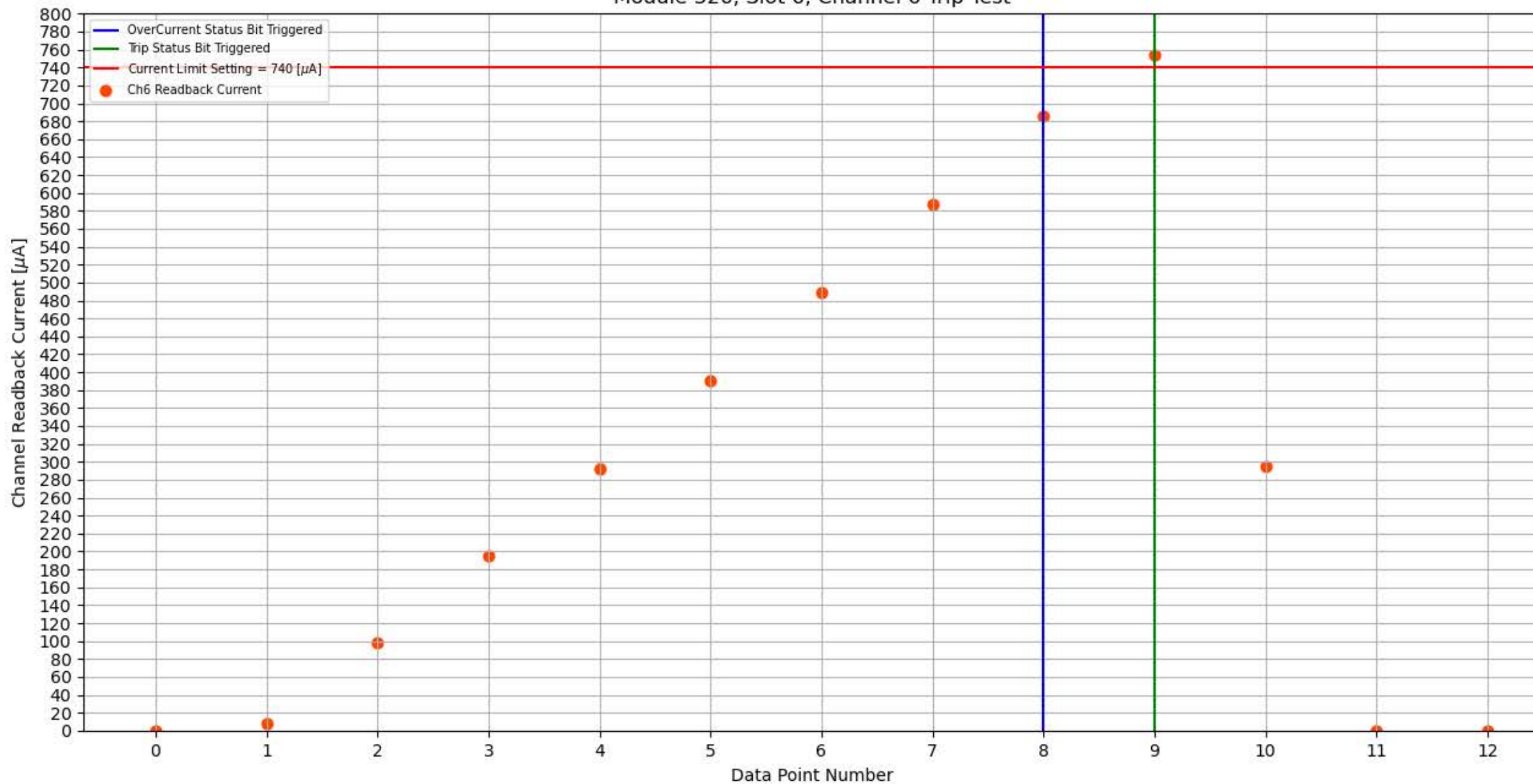
Module 326, Slot 6, Channel 6 Trip Test
