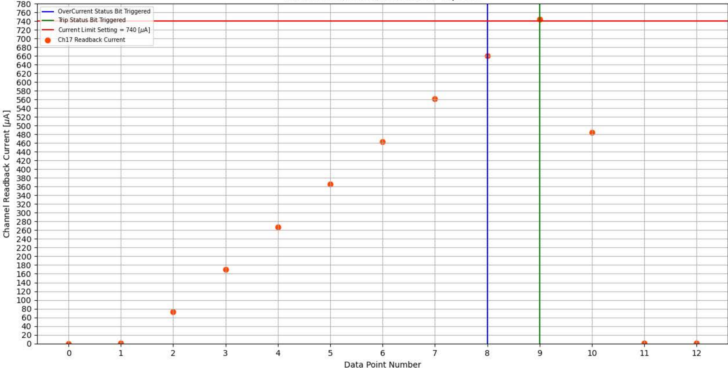
Module 326, Slot 6, Channel 17 Trip Test
