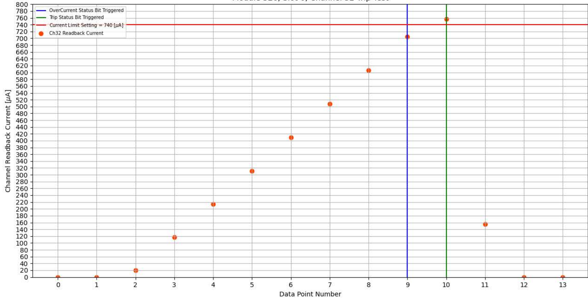
Module 326, Slot 6, Channel 32 Trip Test
