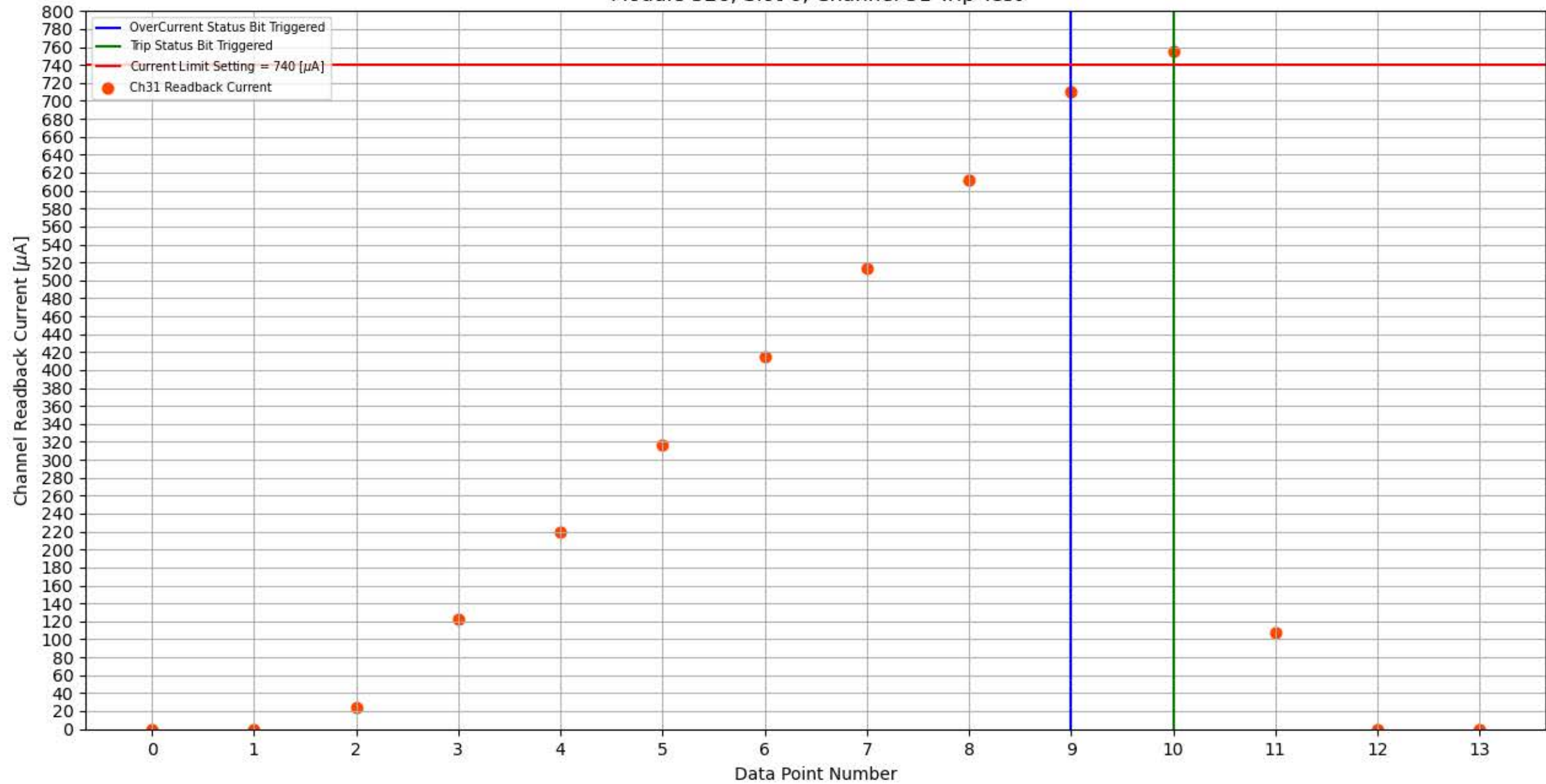
Module 326, Slot 6, Channel 31 Trip Test
