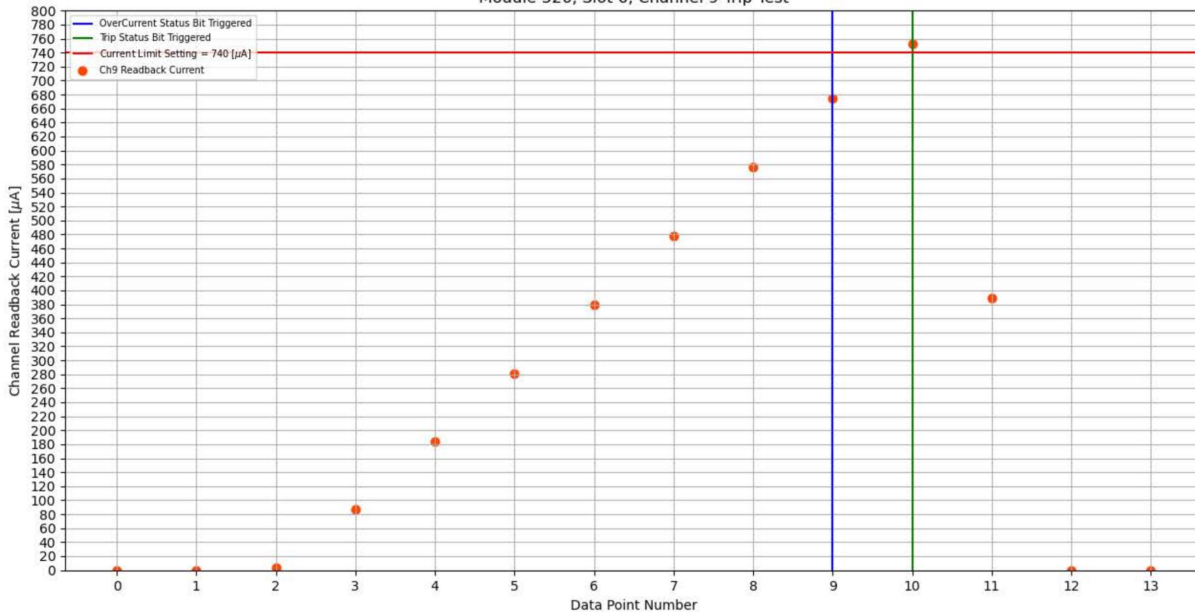
Module 326, Slot 6, Channel 9 Trip Test
