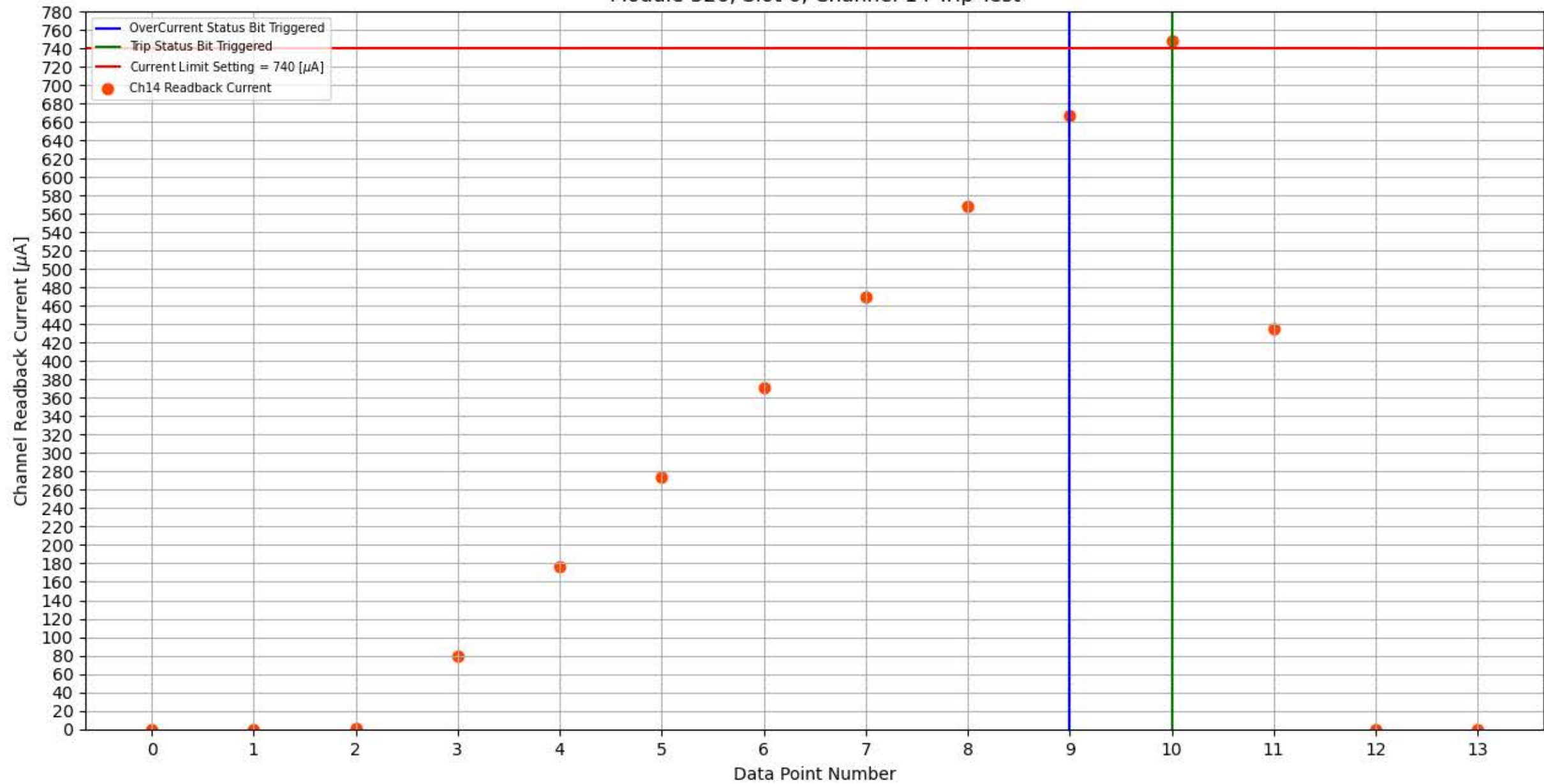
Module 326, Slot 6, Channel 14 Trip Test
