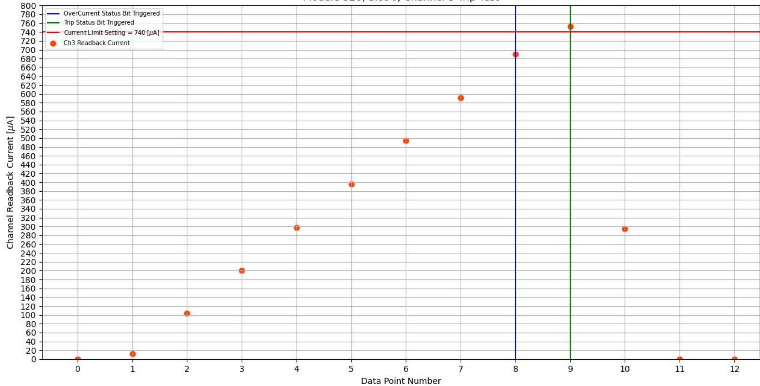
Module 326, Slot 6, Channel 3 Trip Test
