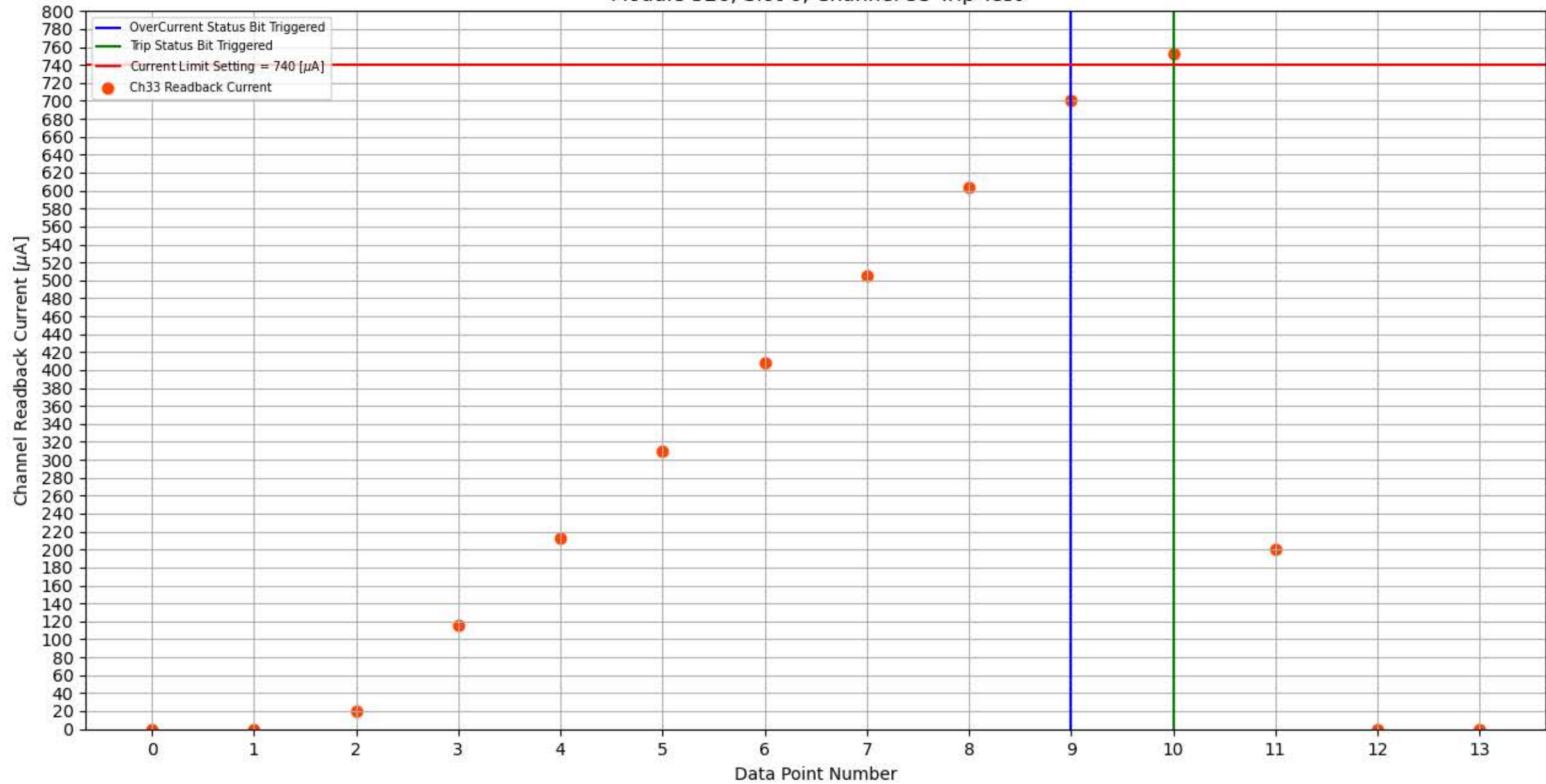
Module 326, Slot 6, Channel 33 Trip Test
