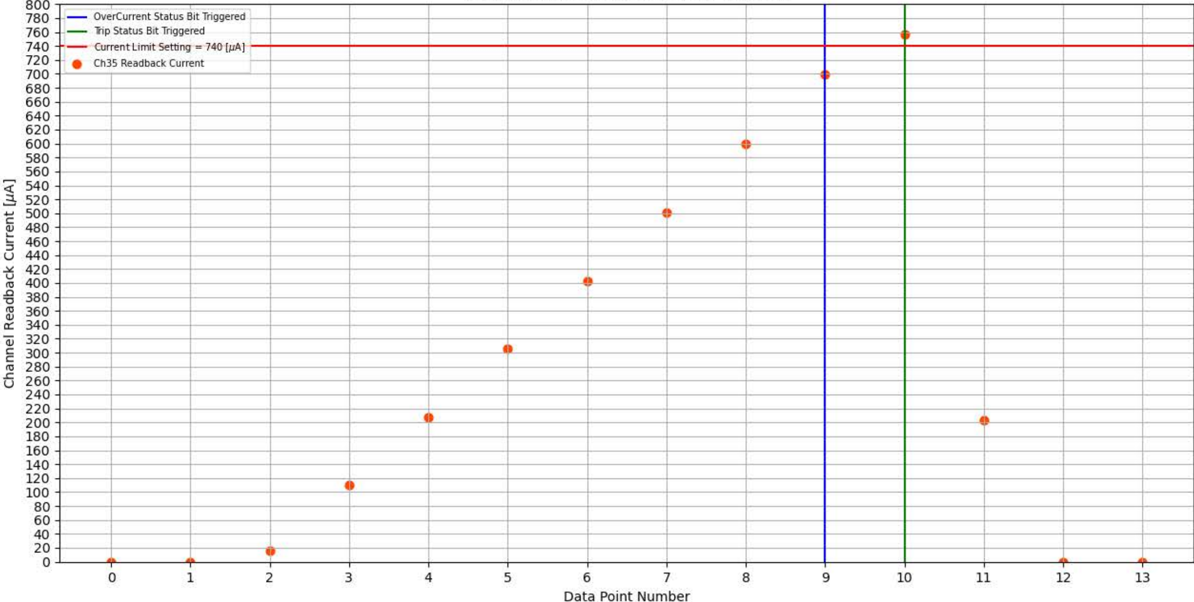
Module 326, Slot 6, Channel 35 Trip Test
