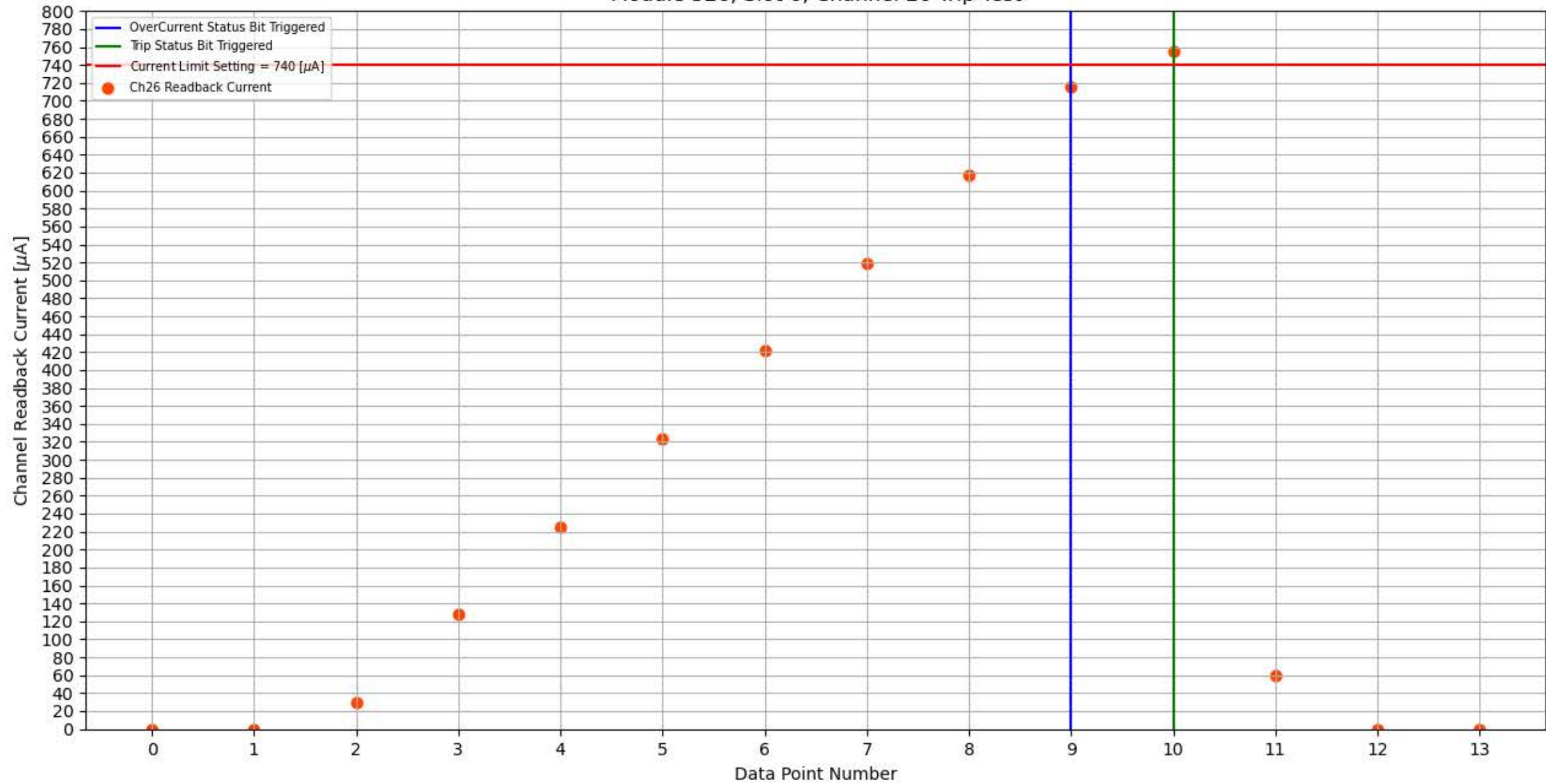
Module 326, Slot 6, Channel 26 Trip Test
