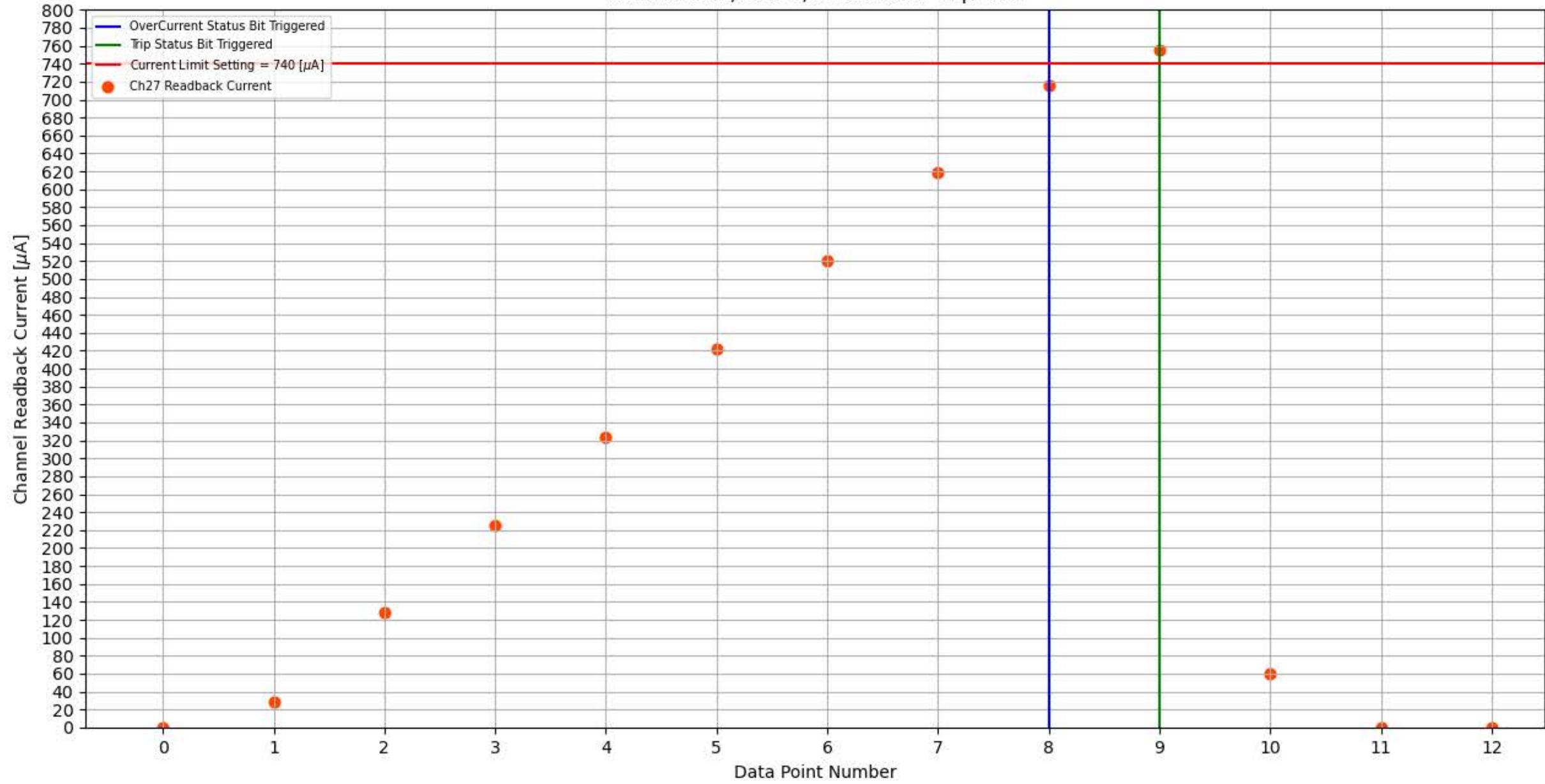
Module 326, Slot 6, Channel 27 Trip Test
