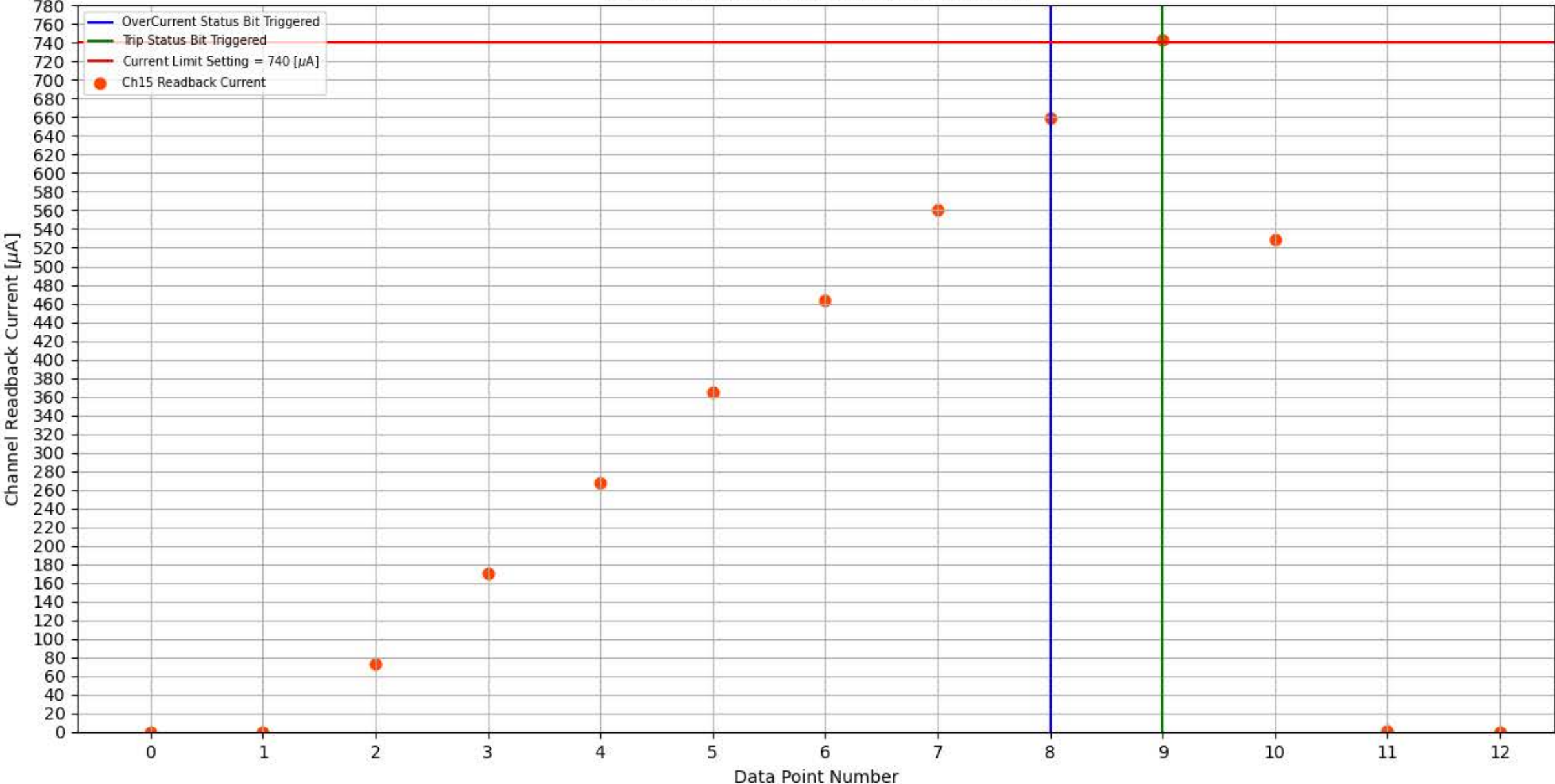
Module 326, Slot 6, Channel 15 Trip Test
