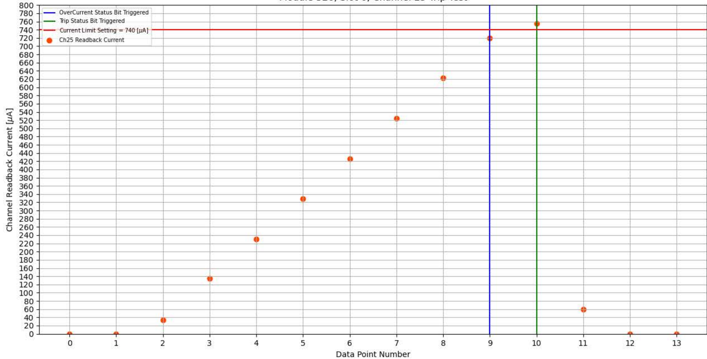
Module 326, Slot 6, Channel 25 Trip Test
